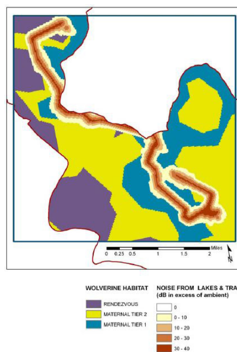
Figure 6: An example of using the SPreAD model to identify the overlap of snowmobile noise emissions and wolverine habitat types (Reed et al. 2009).
